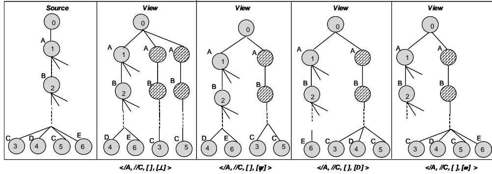
Figure 4. Selective sibling decorrelation examples
