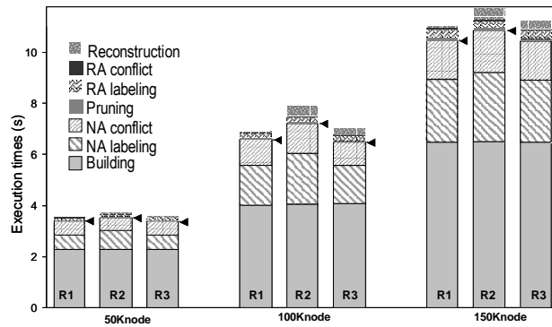
Figure 6. Impact of RA on the motivating example.
