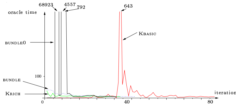
Figure 7: CVRP: oracle computing time for instance E-m22-N4
