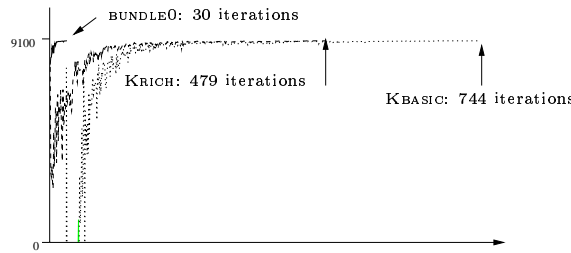
Figure 8: TSP: results with bays29
