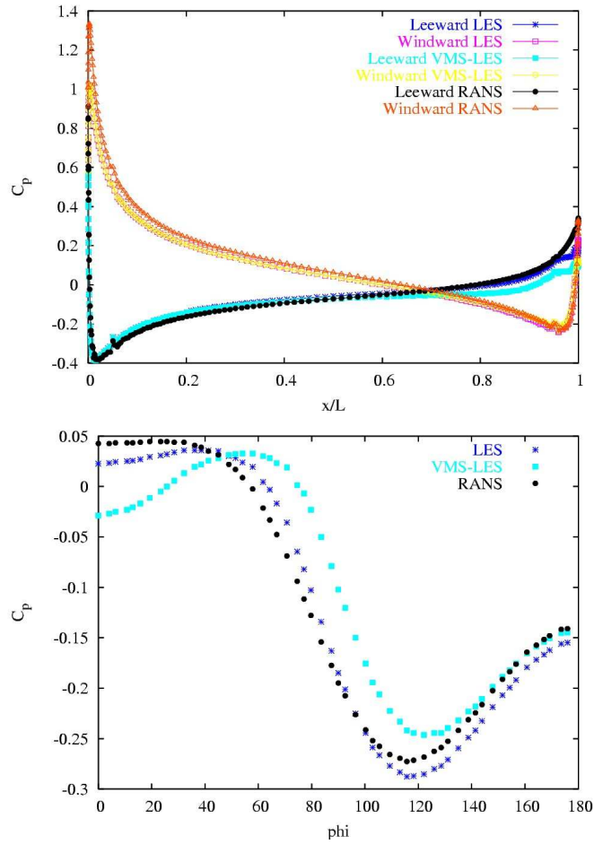
Figure 5: Pressure Coefficient C_p on the prolate surface at z = 0 (top) and at x = 1.2 m (bottom)
