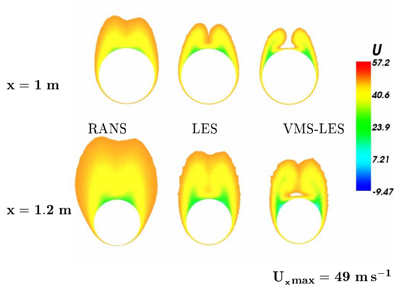
Figure 3: Streamwise velocity isovalues on cross-planes at x = 1 \text{ m} and x = 1.2 \text{ m}
