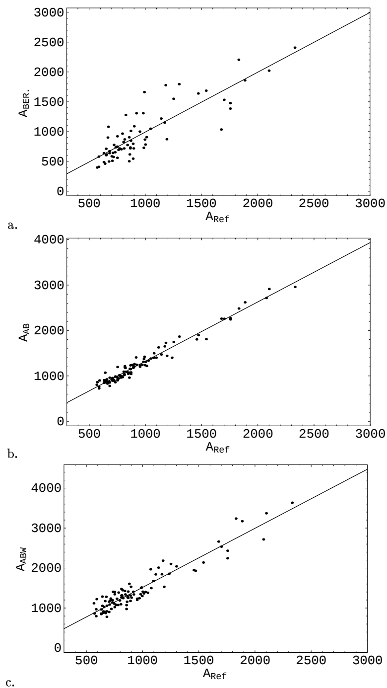
Figure 14: Linear correlations between area values : (a) A_{BER} VISA vs A_{Ref} . SASL (b) A_{AB} vs A_{Ref} . SASL (c) A_{ABW} vs A_{Ref} . SASL
