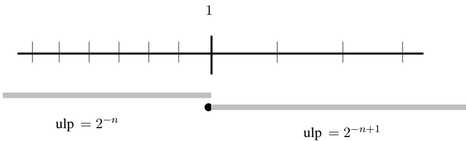
Figure 4: The values of \text{Modified GoldbergUlp}(x) near 1, assuming a binary FP system with n -bit mantissas. Notice that \text{Modified GoldbergUlp}(x) and \text{HarrisonUlp}(x) only differ when x is a power of the radix.
