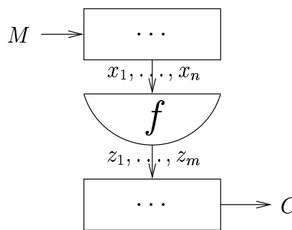
Block Cipher
