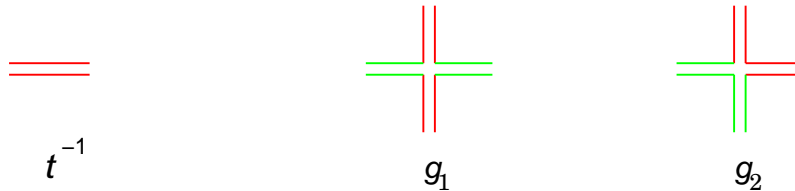
FIGURE 6. The three coupling constants
