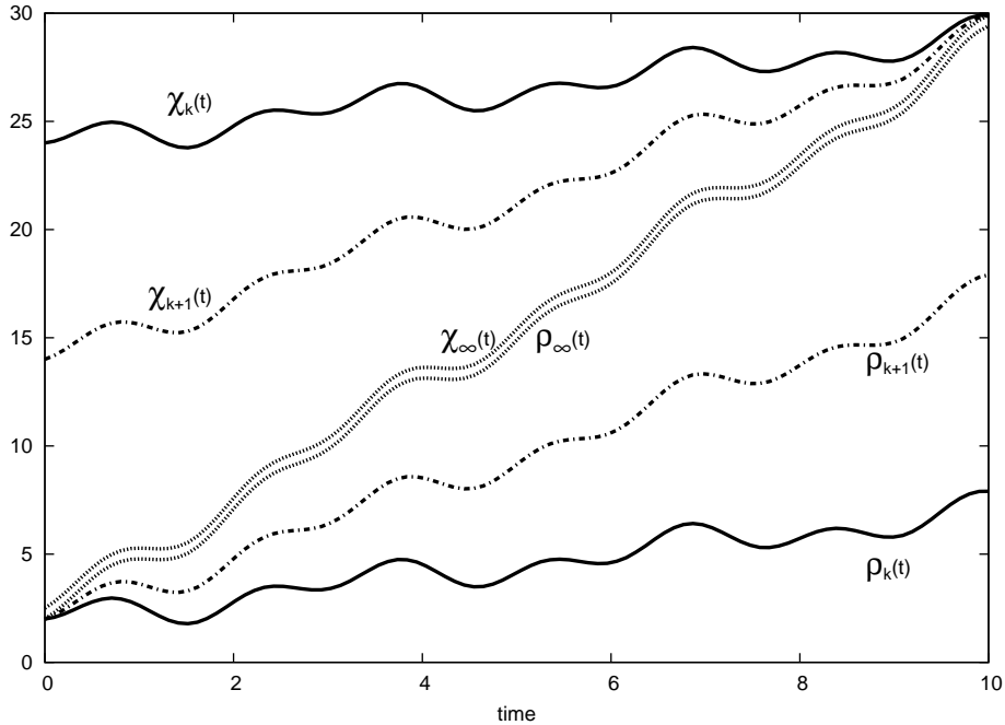
FIG. 1 – Schematic illustration of the convergence of the monotonic algorithms for negligible fluence. The evolving state \rho_{k+1} is approaching monotonically the reference trajectory \chi_k . At the next iteration \chi_{k+1} will remain at a constant distance from \rho_{k+1} because both use the same field \epsilon_{k+1} . This shrinking distance between the two trajectories ensure the progression of the cost functional toward optimal values. This observation is currently used in the context of efficient parallelization of the numerical resolution of quantum control problems [25]. In the general case, the decreasing character of the distance between the curves is weighted by the field fluence and the optimal couple of trajectories will be a tube whose nonzero width is related to the driving laser field fluence.
