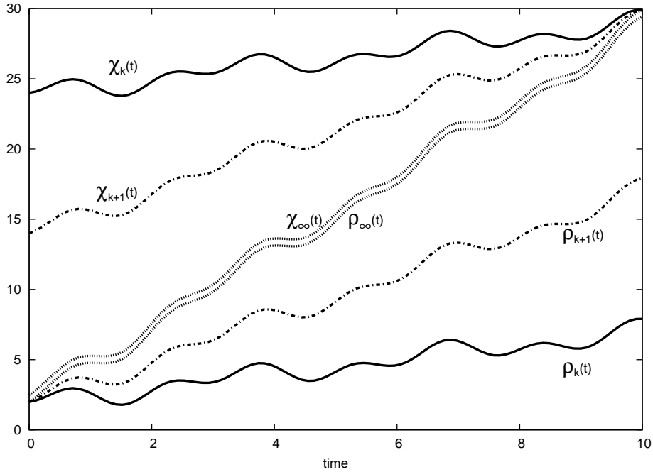
FIG. 1 – Schematic illustration of the convergence of the monotonic algorithms for negligible fluence. The evolving state \rho_{k+1} is approaching monotonically the reference trajectory \chi_k . At the next iteration \chi_{k+1} will remain at a constant distance from \rho_{k+1} because both use the same field \epsilon_{k+1} . This shrinking distance between the two trajectories ensure the progression of the cost functional toward optimal values. This observation is currently used in the context of efficient parallelization of the numerical resolution of quantum control problems [25]. In the general case, the decreasing character of the distance between the curves is weighted by the field fluence and the optimal couple of trajectories will be a tube whose nonzero width is related to the driving laser field fluence.
