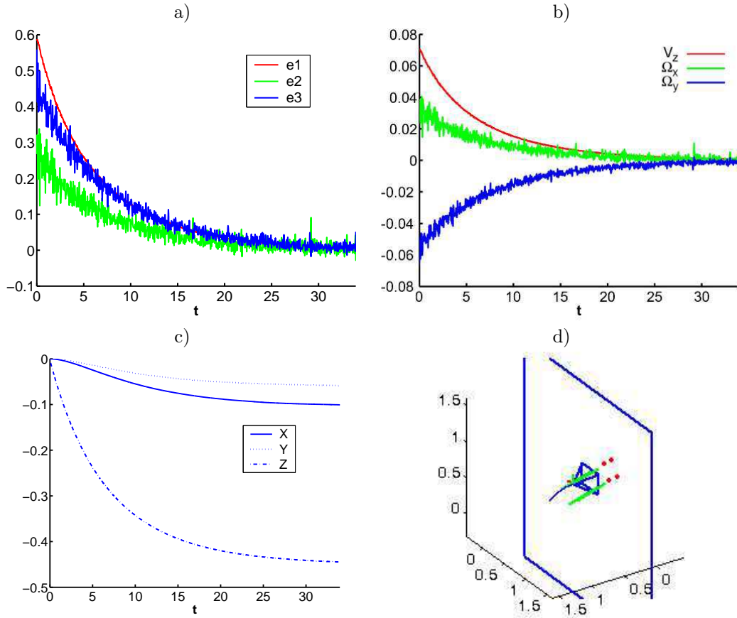
Figure 11: System including large laser-cross misalignment and image noise: simulation using \mathbf{s} = (\gamma, \beta, \alpha) and the constant control law. a) \mathbf{e} = \mathbf{s} - \mathbf{s}^* vs. time (in s). b) Camera velocities (ms/s and rad/s) vs. time. c) Fixed point coordinates in the camera frame. d) Scheme of the camera trajectory.
