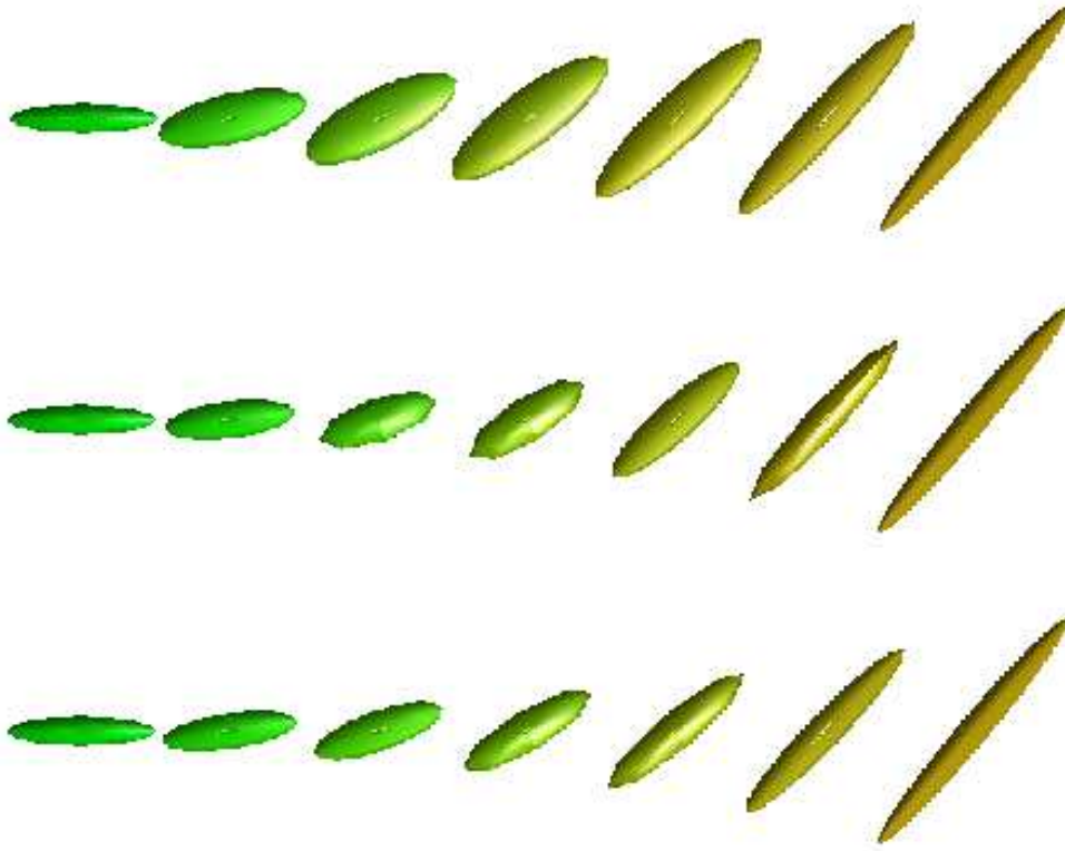
Figure 1: Linear interpolation of two tensors. Above: linear interpolation on coefficients. Middle: affine-invariant interpolation. Below: Log-Euclidean interpolation. Note the characteristic swelling effect observed in the Euclidean case, which is not present in both Riemannian frameworks. Note also that Log-Euclidean means are more anisotropic their affine-invariant counterparts.
