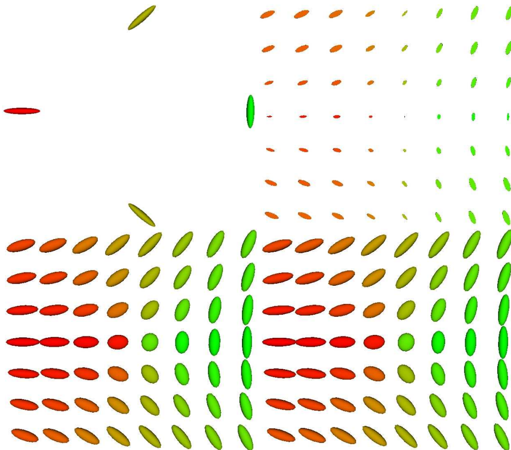
Figure 3: Dense extrapolation of tensors with harmonic diffusion. Upper Left: germs. Upper Right: magnified visualization of the absolute value of the Euclidean difference between the two extrapolations. Lower Left: affine-invariant extrapolation. Lower Right: Log-Euclidean extrapolation. Note that the Log-Euclidean extrapolation yields tensors a little more anisotropic. The differences are very small, and are mostly concentrated along the direction of anisotropy.
