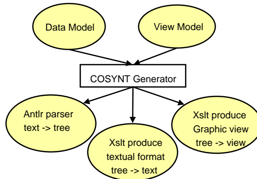
Figure 14: COSYNT generator
