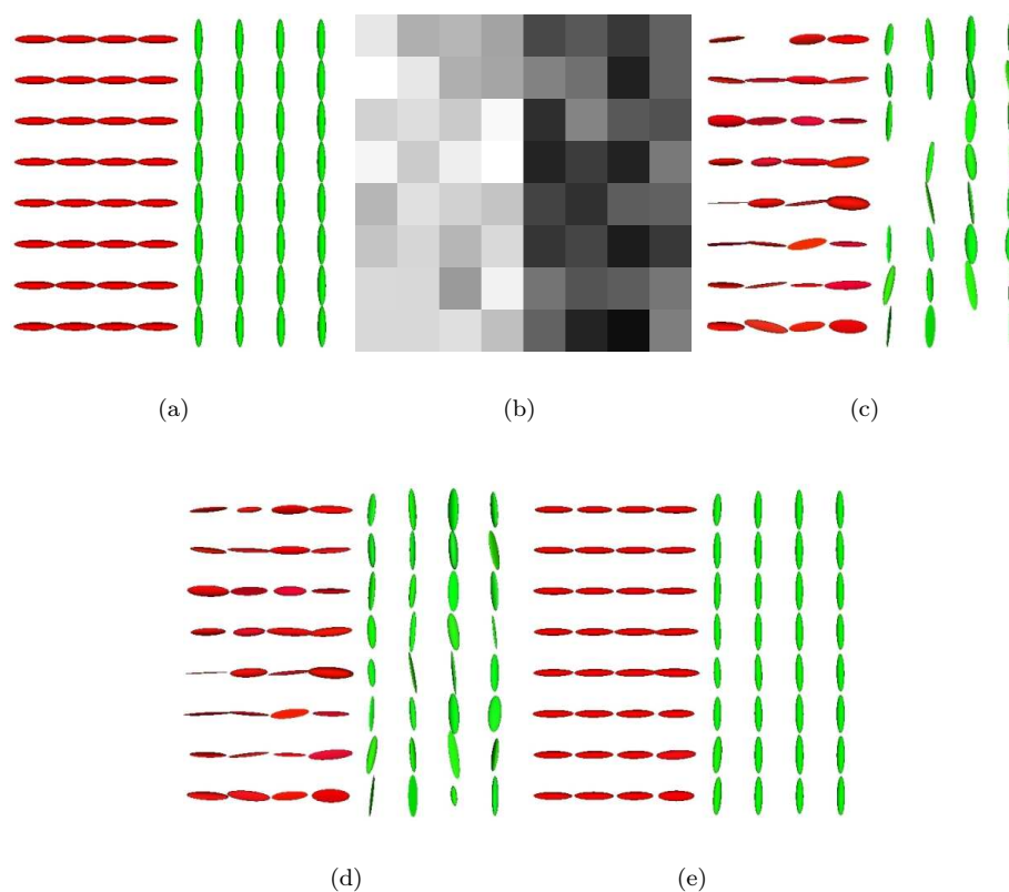
Figure 2: Estimation of the tensor field from the noisy synthetic data. (a): a 2D slice of the 3D synthetic field. (b): a 2D slice of a synthetic DWI (gradient: (0,1,0) ) + noise, (c): the classical estimation, (d): the LSQ on DTI intensities, (e): the LSQ + regularization.
