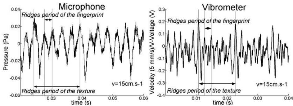
Figure 8. Teeth moving forward, v=15\text{cm}\cdot\text{s}^{-1}
