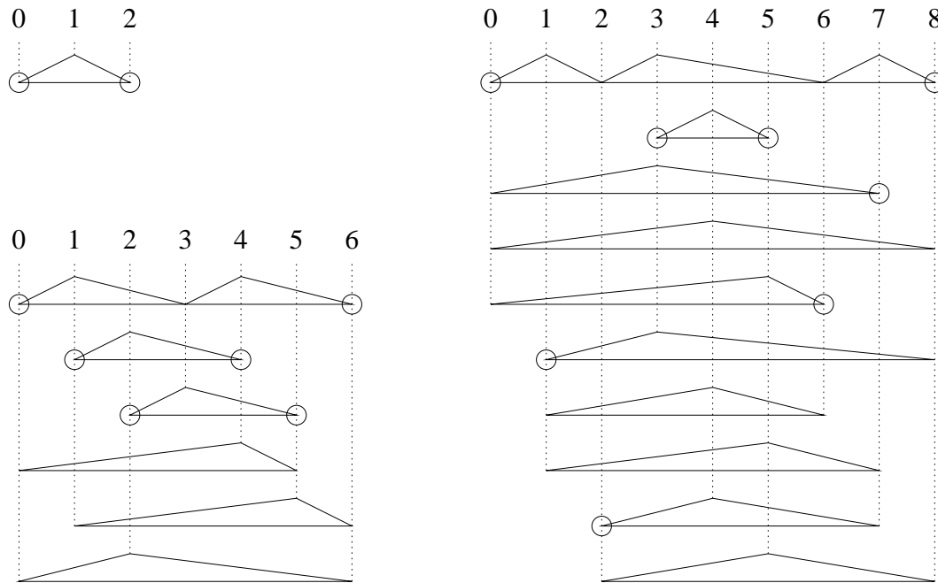
Figure 3: Construction for N = 3, 7 and 9 . Left and right most nodes have been circled.
