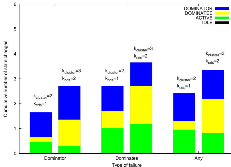
Figure 16: Number of changes of cds-states after a discrete movement
