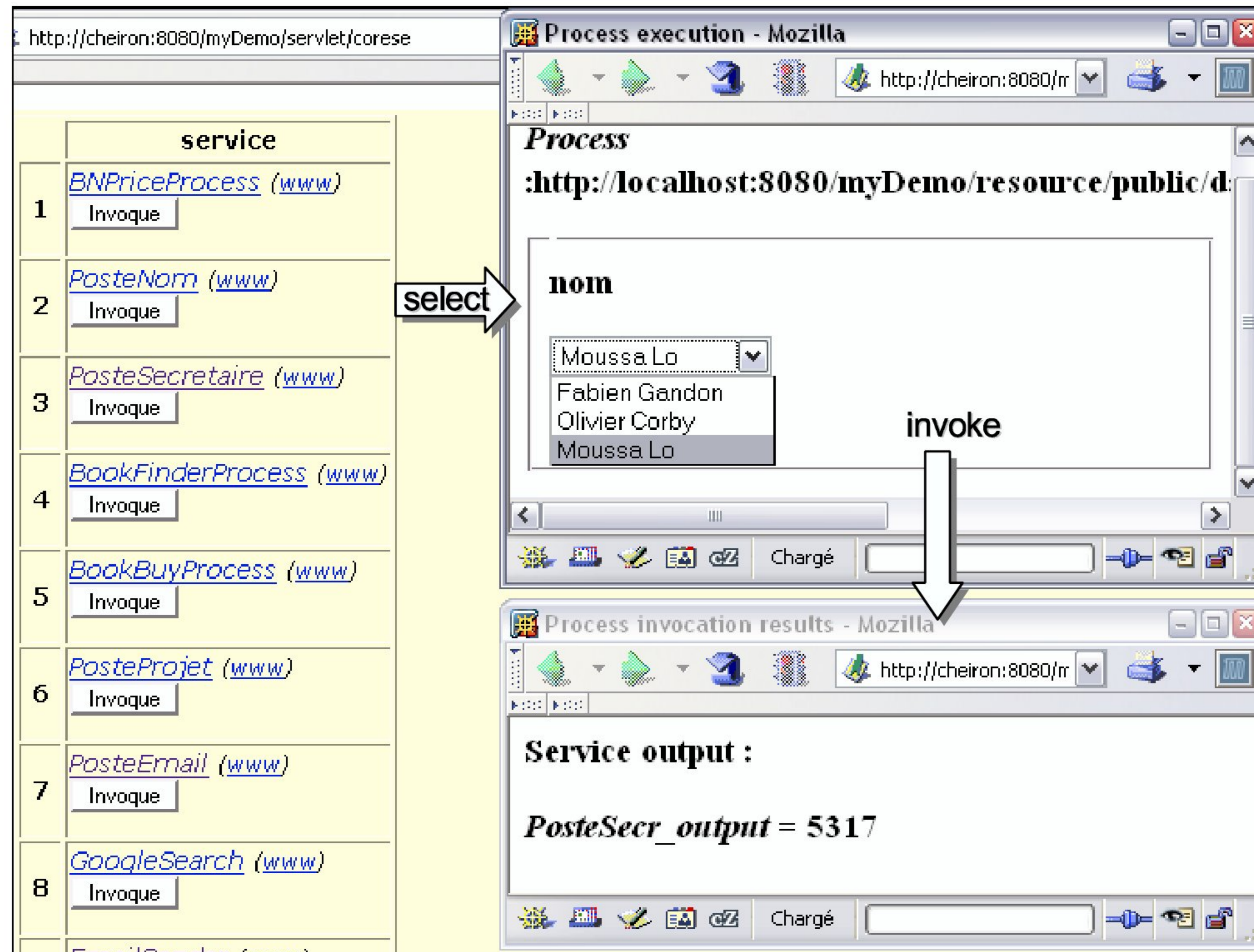
Figure 16. Leveraging the corporate memory to populate a SWS input
