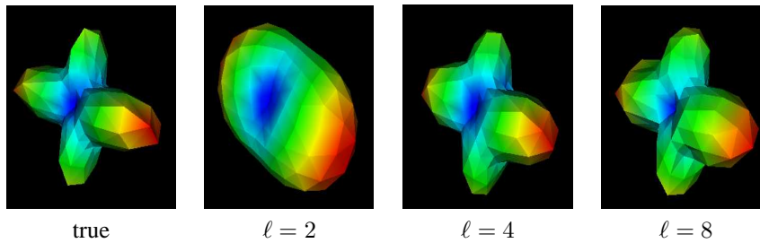
Figure 9: Rank-2 approximation fails to describe non-Gaussian diffusion.
