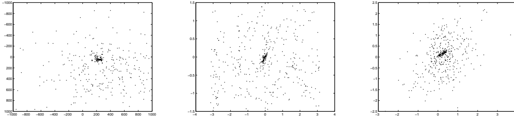
Figure 15: ‘‘Guernica experiment: Each point represents a transformation associated with an affine invariant meaningful match, described by 6 parameters. Each figure represents a two-dimensional projection of the points, respectively t_x vs. t_y (translation coordinates), \theta (rotation) vs. \varphi (shear), and \ln(s_x) vs. \ln(s_y) (zooms in the x and y directions). The noise is mainly due to global shape elements that are very much alike up to affine transformations, and which do not belong to the same real shape. The main cluster is also spread because of the effect of perspective.
