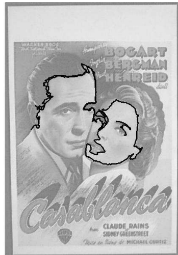
(b) Second maximal meaningful group: 7 meaningful matches, -\log_{10}(NFA_g) = 6.62
