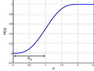
Figure 5: The function H with \rho_H = 1 .
