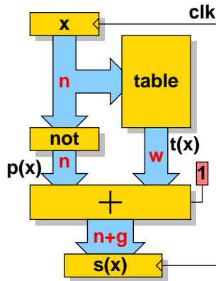
Figure 3: Architecture of the seed generator.
