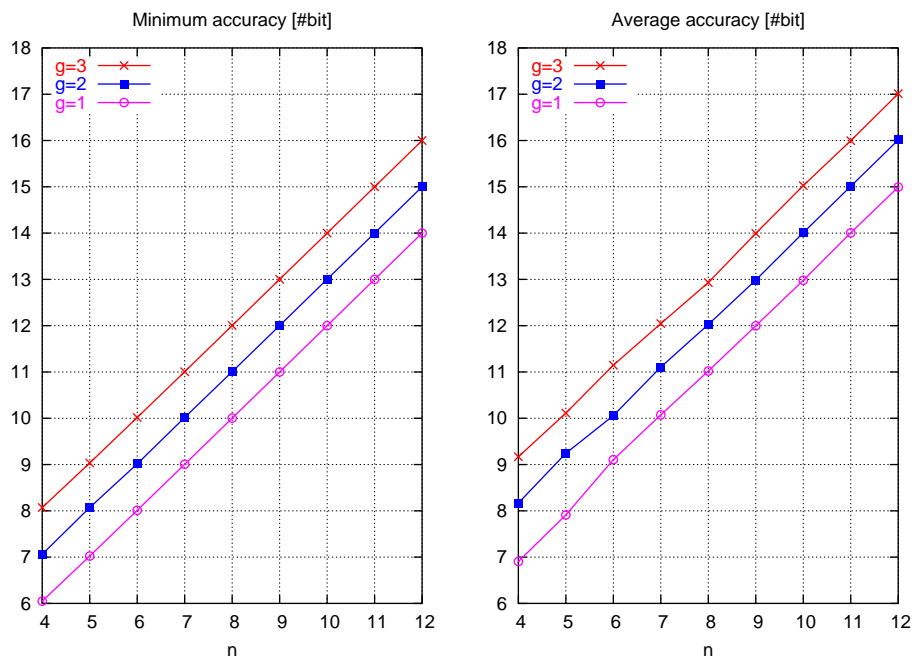
Figure 10: Maximum and average accuracy obtained for the reciprocal.
