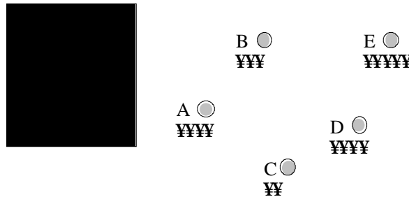
Figure 2 A five node Joyce group and its multi-log representation on A.
