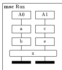
Fig. 4. A run as defined as a bMSC with inline references.
