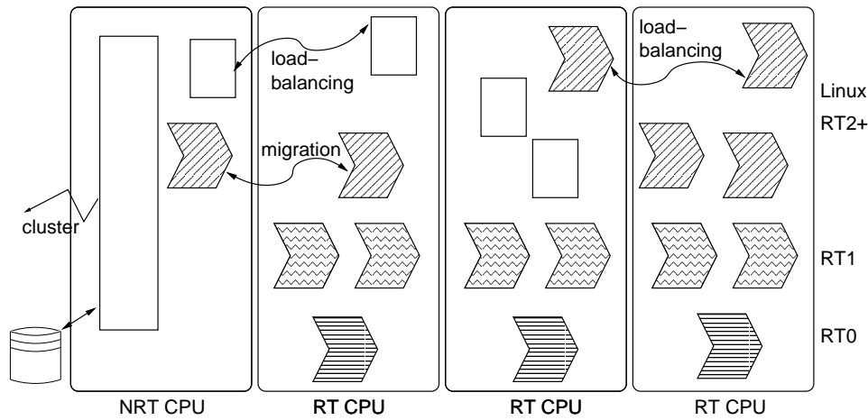
Figure 6: Mapping of the tasks on the RT and NRT processors.
