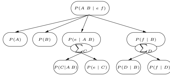
Figure 3: The evaluation tree corresponding to Equation 3.
