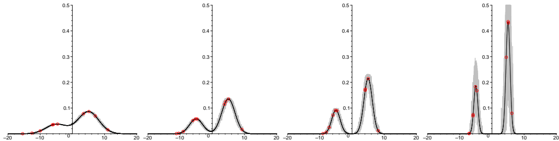
Figure 10: The “temperature reduction” phase of the MCSEM algorithm. In black, the theoretical distribution to maximize and in gray, the estimated one using Monte Carlo numerical integration. From left to right, the T (temperature) parameter is decreased to obtain the original distribution (i.e., T = 0.0 ).
