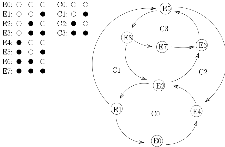
Fig. 6.4: Graph of the state space for a TASEP with three particles and the dual graph corresponding to the possibles cycles.
