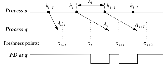
Figure 9: Failure detection with the heartbeat strategy
