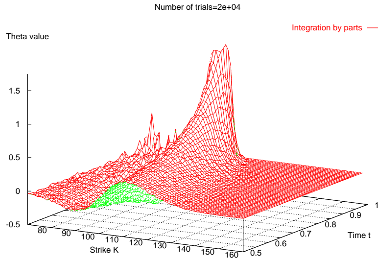
Figure 4 : Theta as a function of t and K by integration by parts
