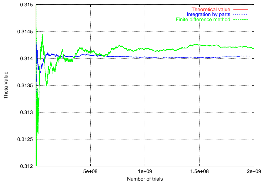
Figure 2 : Estimation of Theta vs number of trials
