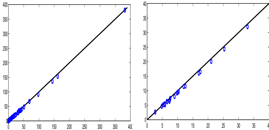
Figure 4: Connectivities between groups ( A_{qe} : left) and mean degree ( \lambda_q : right). x -axis = expected, y -axis = 'observed'
