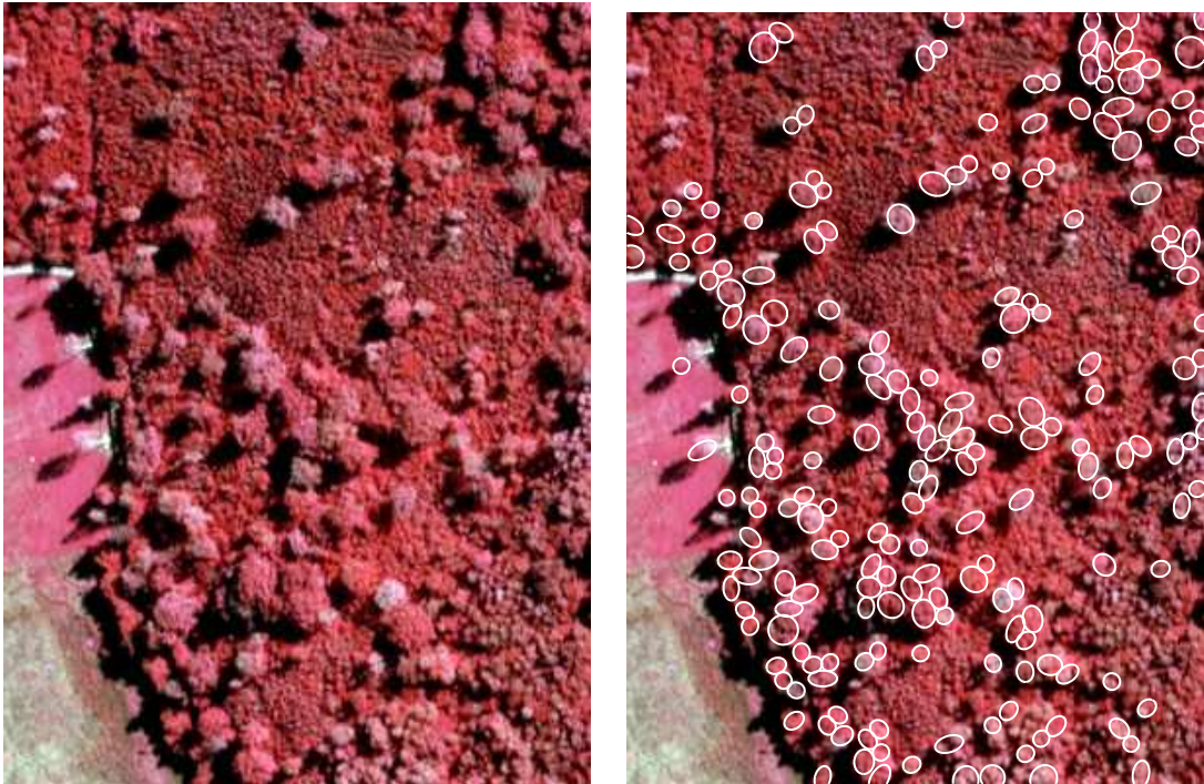
Figure 18: Left : 300 \times 400 image of mixed height stands ©IFN. Right : extraction result, 5 millions of iterations ©INRIA.
