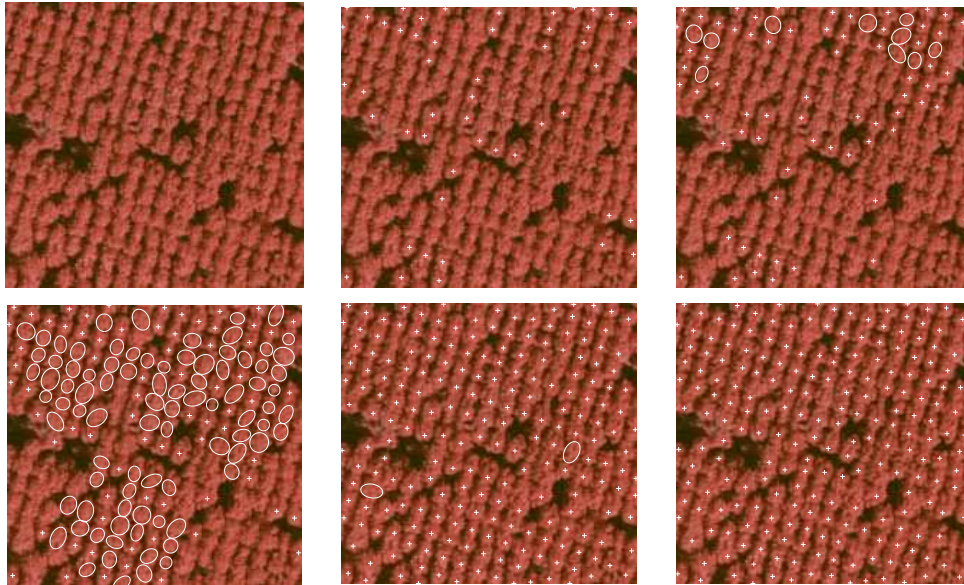
Figure 12: Top left : original image ©IFN. Top middle : 2D model without correction, \left| \frac{\gamma_p}{\gamma_d} \right| = 0 (49 objets). Top right : 2D model without correction, \left| \frac{\gamma_p}{\gamma_d} \right| = 0.1 (79 objets). Bottom left : 2D model without correction, \left| \frac{\gamma_p}{\gamma_d} \right| = 0.2 (159 objets). Bottom middle : 2D model with correction, \left| \frac{\gamma_p}{\gamma_d} \right| = 0.1 and p_{2D} = 10\% (214 objets). Bottom right : 2D model with correction, \left| \frac{\gamma_p}{\gamma_d} \right| = 0 and p_{2D} = 15\% (217 objets). For all result images ©INRIA. For more visibility, extracted objects with a negative data energy are represented by crosses, while extracted objects with a positive data energy (which have been accepted thanks to the prior term) are represented by ellipses.
