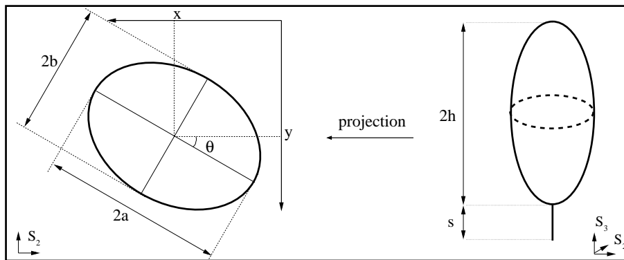
Figure 1: Left : position and marks of an ellipse of S_2 . Right : additional mark for an ellipsoid of S_3 .
