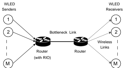
Figure 3: Simulation topology.
