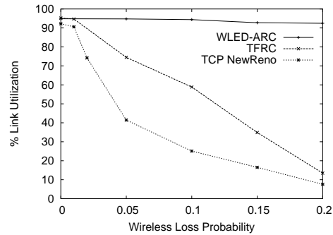
Figure 6: Link Utilization for Different Wireless Loss Probabilities.
