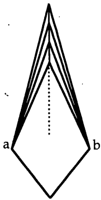
(A) \rightarrow\text{U}(X) complete
