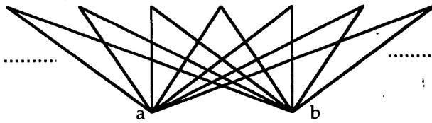
(B) \rightarrow\text{U}(X) finite
