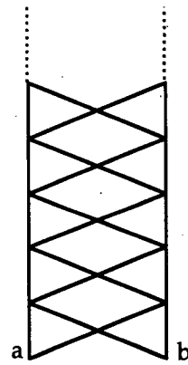
(C) \rightarrow\text{U}^*(X) finite \square
