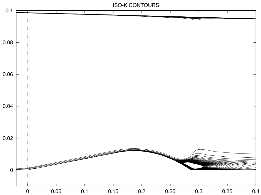
Figure 26: Transonic Bump Flow: M_\infty = 0.635 , Re_\infty = 1.3510^7 Navier-Stokes Computation, iso-k lines (partial view)
