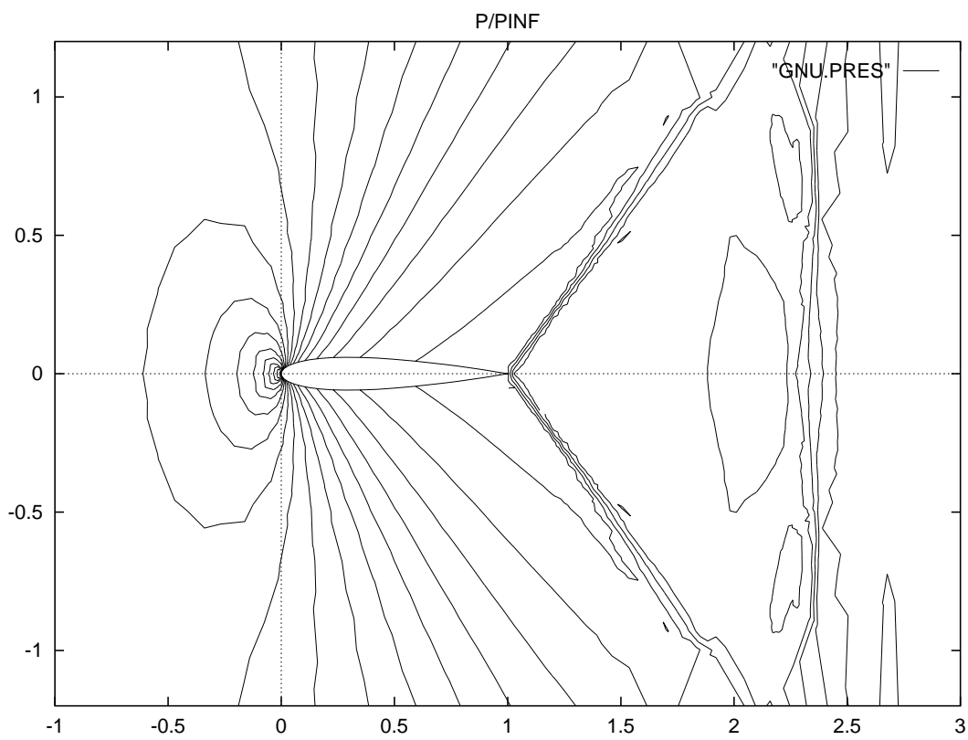
Figure 17: NACA 0012, The Fish Tail: M_\infty = 0.95 , Euler Computation, iso-pressure lines (partial view)
