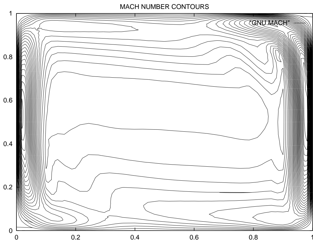
Figure 15: Natural Convection in Square Cavity: Ra = 6 \cdot 10^5 , Mach number contours.
