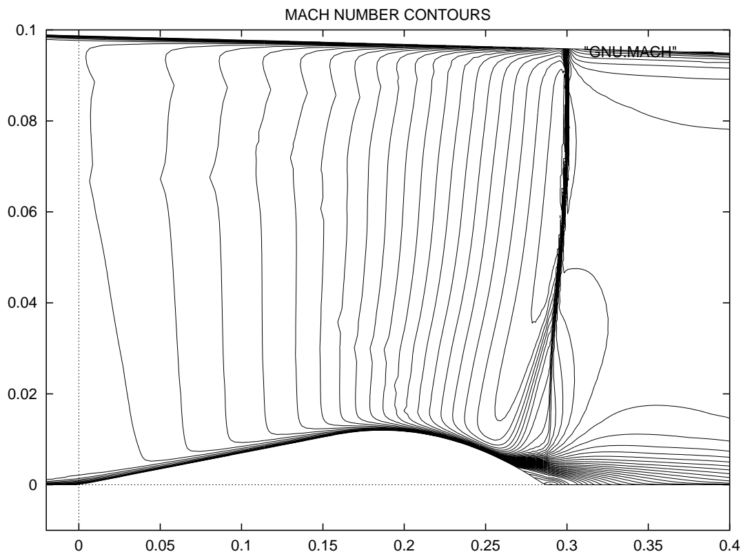
Figure 25: Transonic Bump Flow: M_\infty = 0.635 , Re_\infty = 1.3510^7 Navier-Stokes Computation, iso-Mach lines (partial view)
