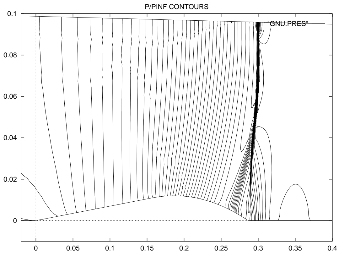
Figure 24: Transonic Bump Flow: M_\infty = 0.635 , Re_\infty = 1.3510^7 Navier-Stokes Computation, iso-pressure lines (partial view)
