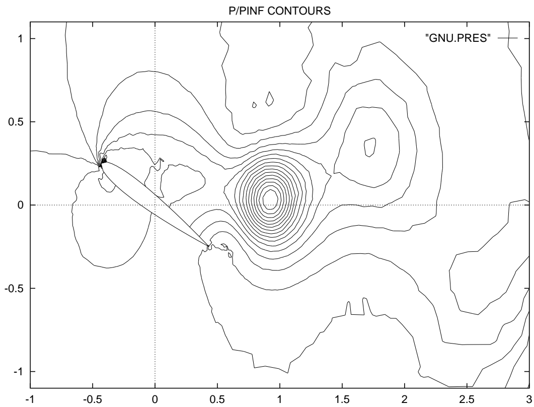
Figure 20: NACA 0012, Unsteady Flow: M_\infty = 0.1 , Re_\infty = 10^6 Navier-Stokes Computation, iso-pressure lines (partial view)
