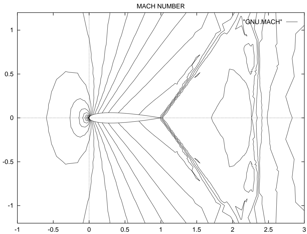
Figure 18: NACA 0012, The Fish Tail: M_\infty = 0.95 , Euler Computation, iso-Mach lines (partial view)
