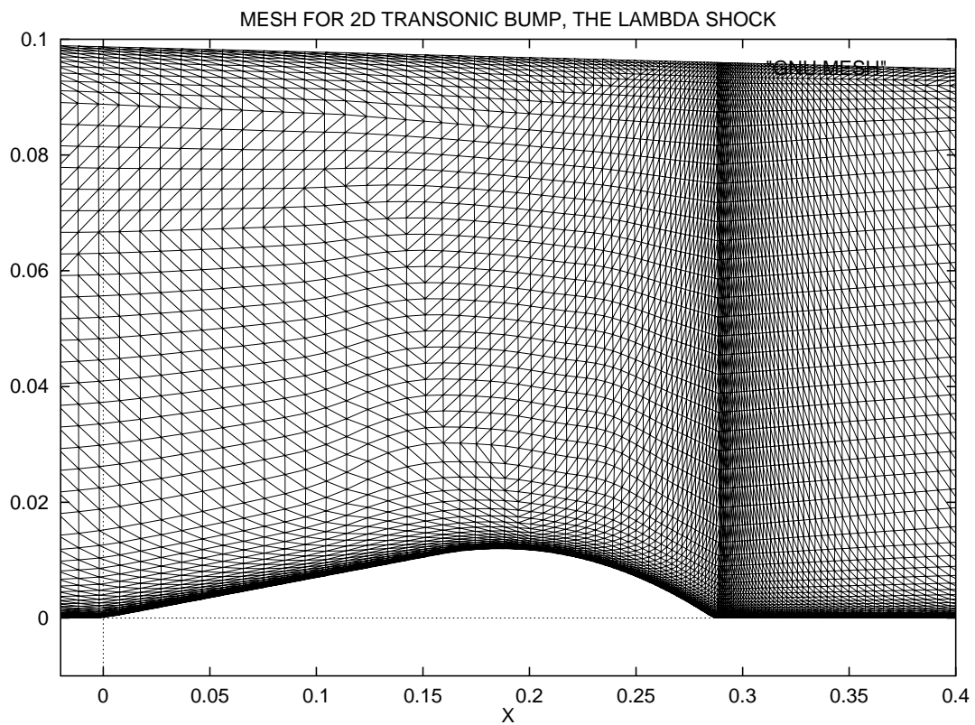
Figure 23: Transonic Bump Flow: M_\infty = 0.635 , Re_\infty = 1.3510^7 , Navier-Stokes Computation, The mesh (partial view)
