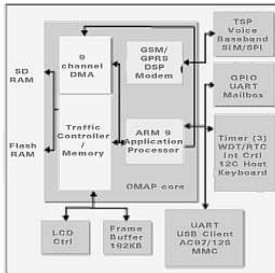
Figure 4.1: Blockdiagramm OMAP710.
