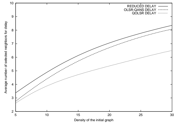
Figure 4: Minimum delay neighbors selection
