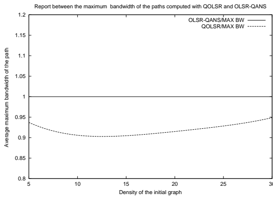
Figure 6: Path average bandwidth comparison
