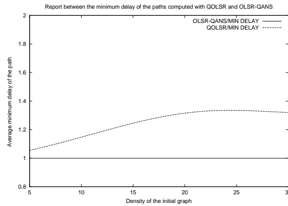
Figure 7: Path average delay comparison
