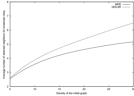
Figure 5: Broadcast forwarding neighbors selection
