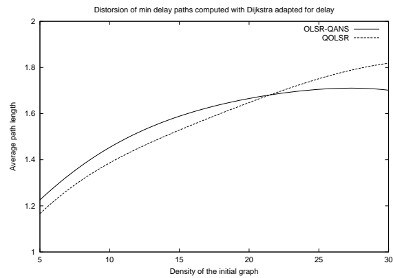
Figure 9: Distorsion of the length of the minimum delay paths
