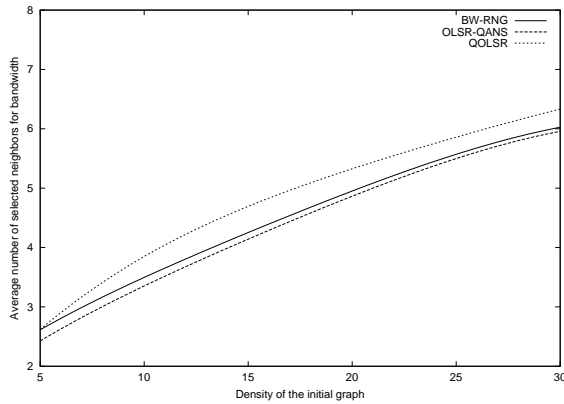
Figure 3: Maximum bandwidth neighbors selection
