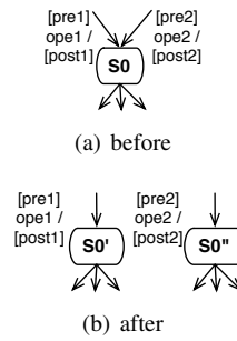
Figure 11. split_state()
