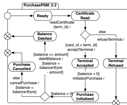
Figure 13. PurchasePSM.5.2
