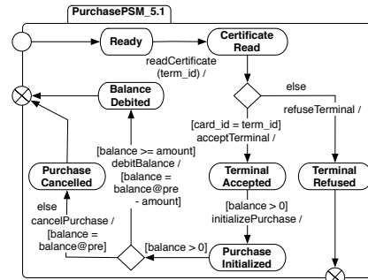
Figure 12. PurchasePSM.5.1
