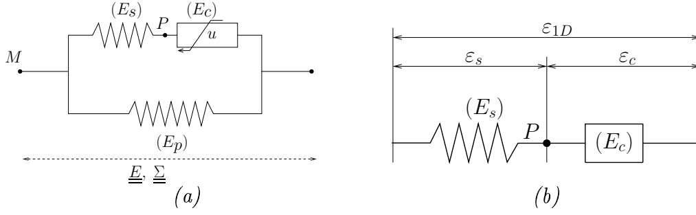
Figure 5: (a) Hill-Maxwell rheological model and (b) strains in the active branch.
