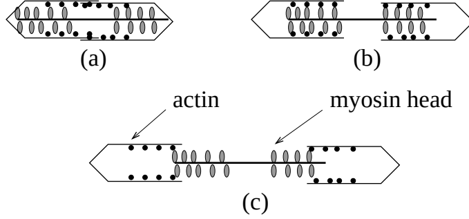
Figure 3: Three different sarcomere deformations.
