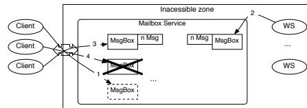
Figure 2. The WS-MsgBox.
