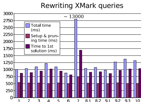
Figure 13: Performance of XMark query rewriting
