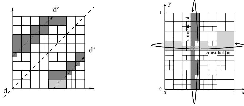
Figure 2: A Thwart Path (left grid) and a Traversal Path (right grid)
