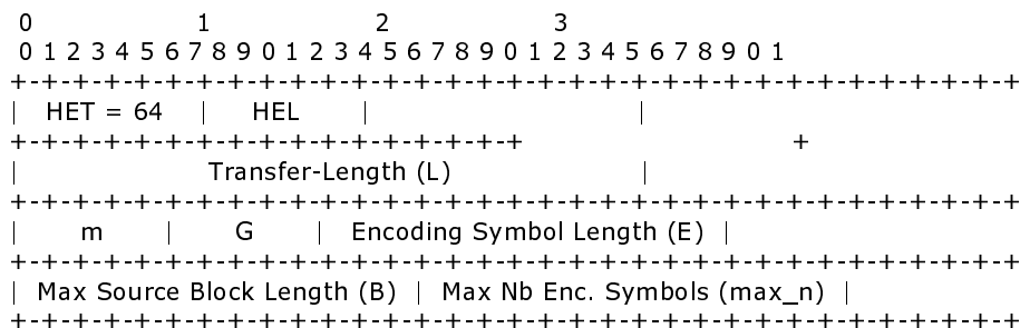
Figure 2: EXT_FT1 Header Format
