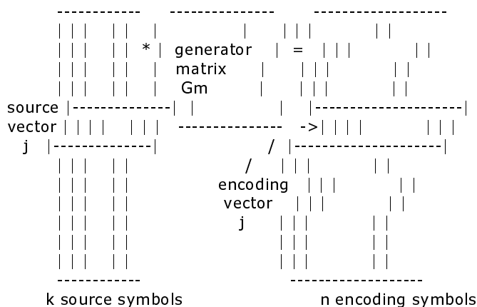
Figure 3: Packet encoding scheme
