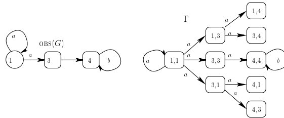
Figure 8: OBS(G_\Omega) and \Gamma for the LTS of Figure 7
