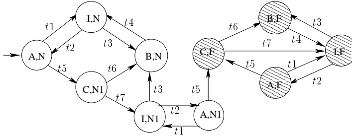
Figure 12: G_\Omega
