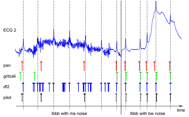
Figure 4: Context transition of ECG 2 with QRS occurrences for each detector. Dotted lines are actual occurrences of QRS.
