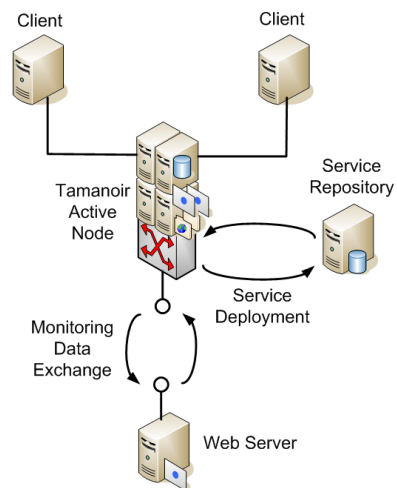
Figure 11: Experimental platform
