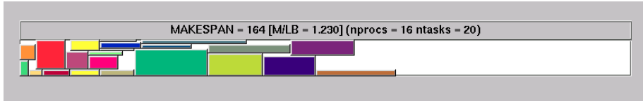
Figure 5: A schedule of 20 tasks on 16 processors with algorithm 3.
