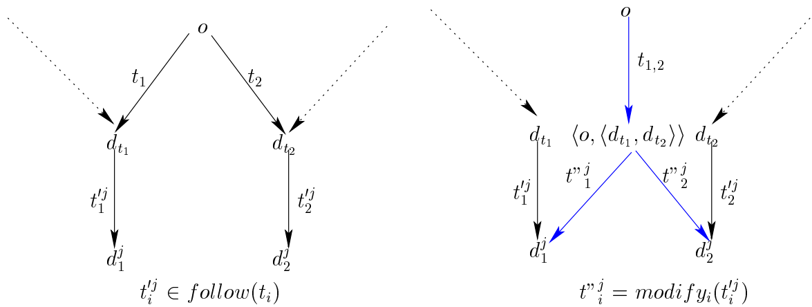
Figure 2: Determinising 2 transitions: (left) before (right) after.
