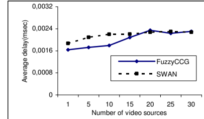
Fig. 7. Average delay in FuzzyCCG and SWAN models vs. number of video flows
