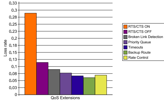
Fig. 11. Loss Rate of Background Traffic - Combined Impact
