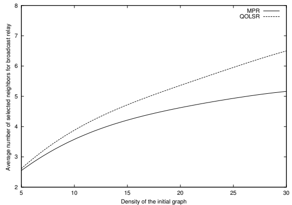
Fig. 4. Broadcast forwarding neighbors selection
