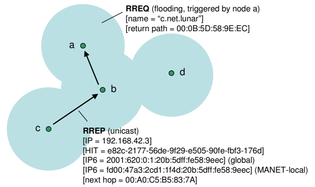
Fig. 6. RREQ/RREP procedure
