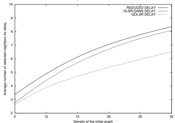
Fig. 5. Minimum delay neighbors selection
